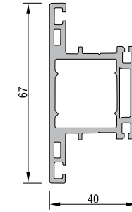
ORTAKAYIT PROFİLİ 21601 - 02000 : BEYAZ
