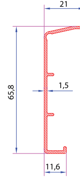
ALM. GİYDİRME NORMAL KASA PRF. ELOKSAL (3900) KODU : 34025 - 28010
