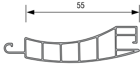
PANJUR LAMEL (55 mm) 20109 - 01100 : BEYAZ
