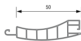
PANJUR LAMEL (50 mm) 20109 - 01000 : BEYAZ
